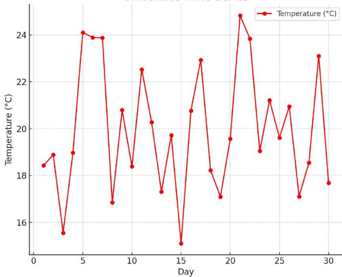
Univariate Time Series
