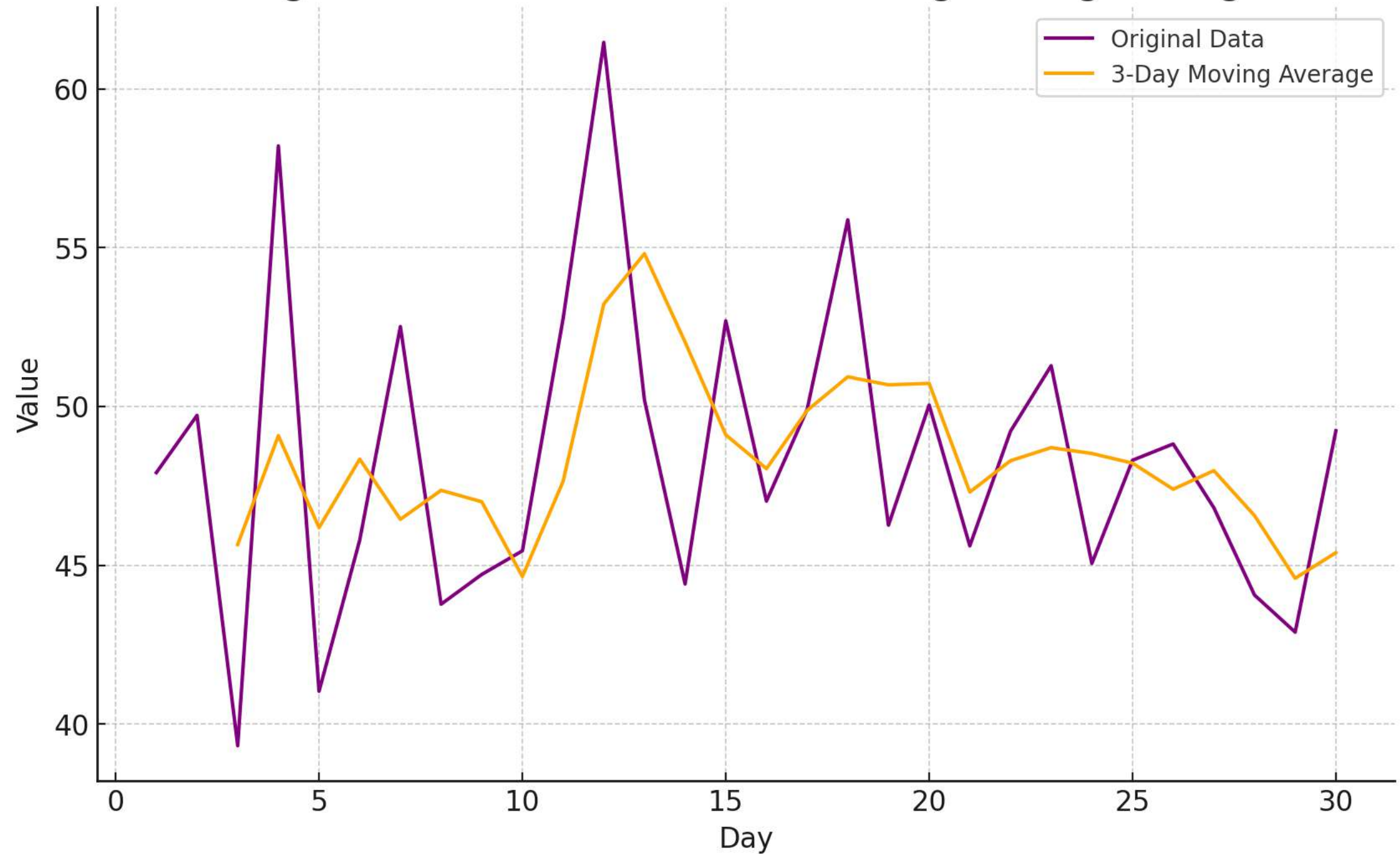
Original Data vs. Smoothed Data using Moving Average
