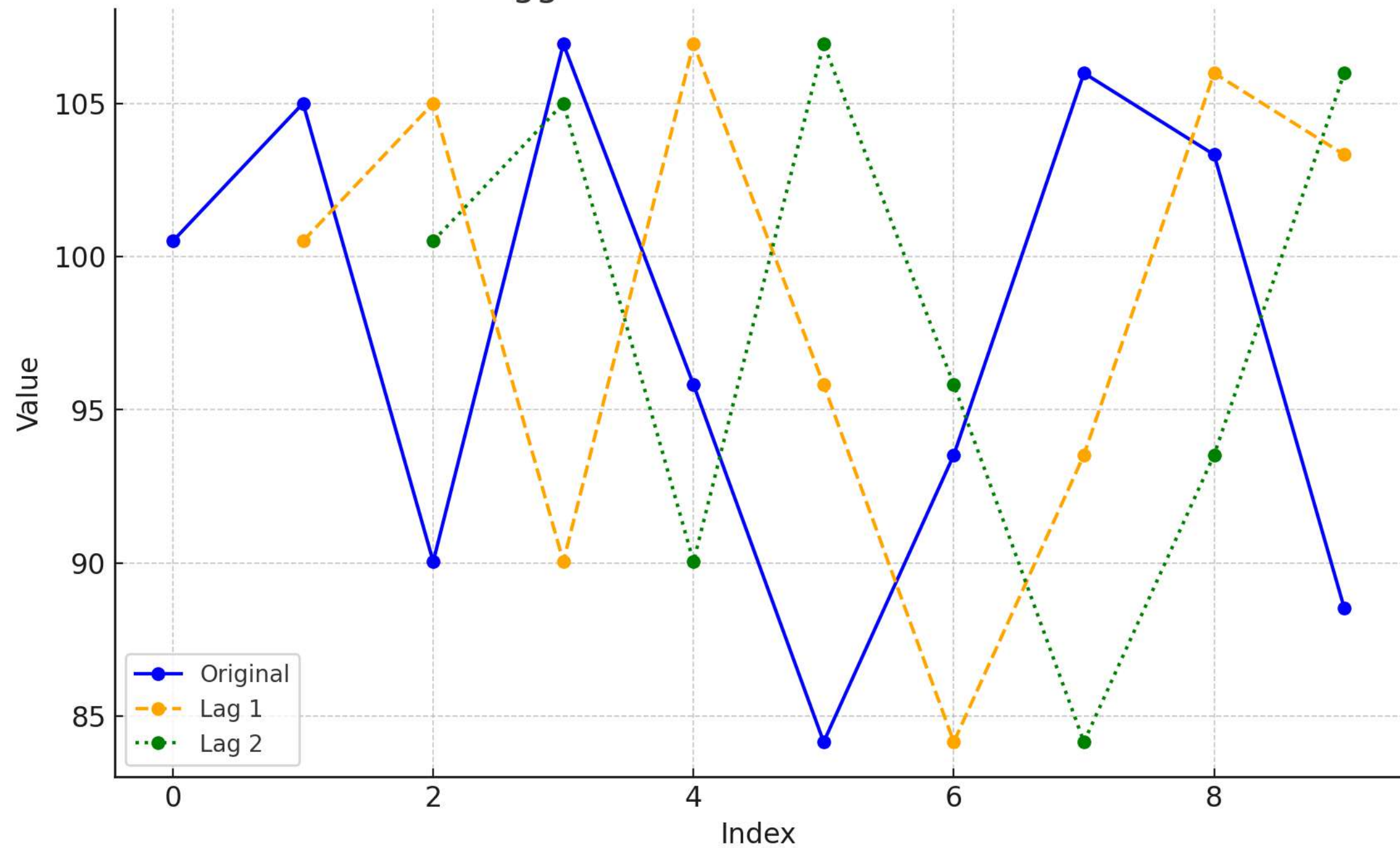
Lagged Features in Time Series
