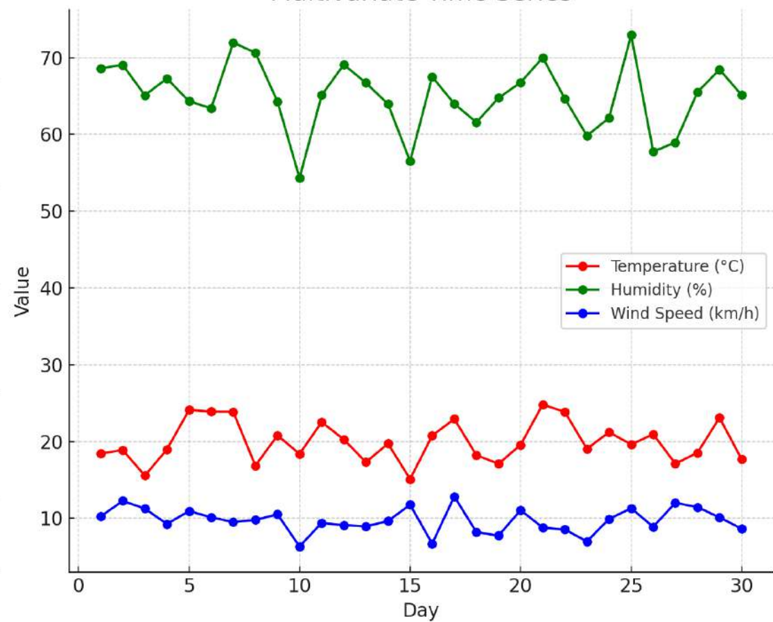
Multivariate Time Series
